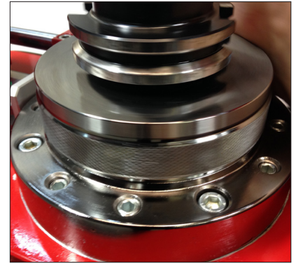
Rotating interchangeable sleeve, with adjustment screws for parallel calibration
